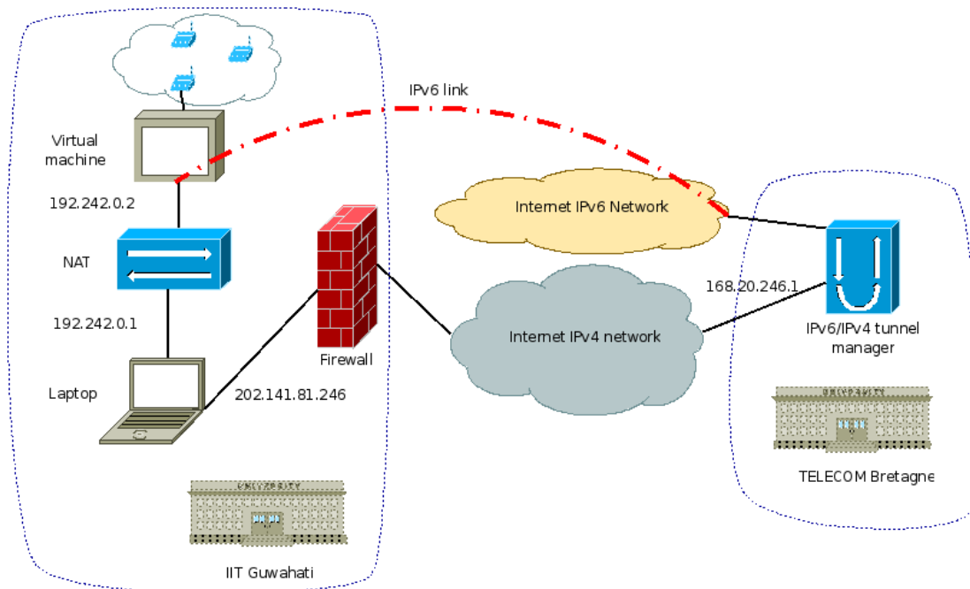
Figure 24. IPv6 Sensor Network (From VieSurIP, n.d.).
